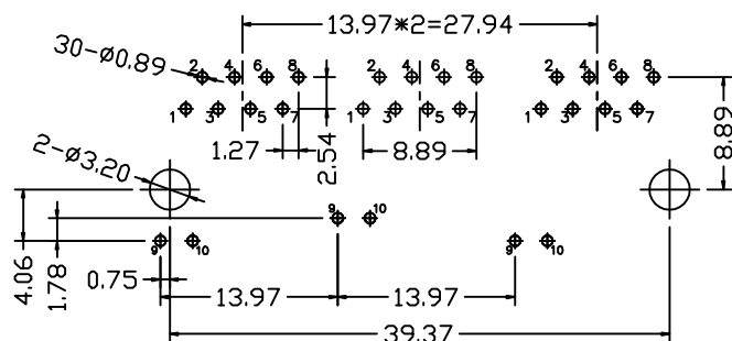
PCB LAYOUT TOP VIEW TOLERANCE:±0.05mm
